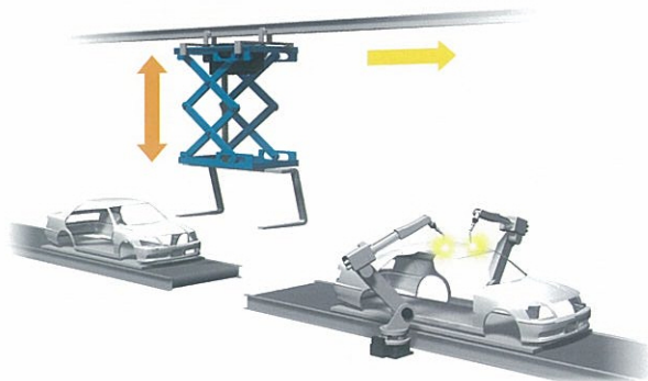
Lifting weight : 1,500kg Stroke : 2,500mm Lift speed : 30m/min
