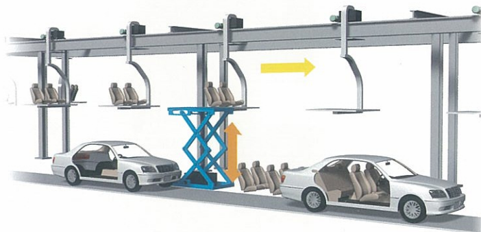
Lifting weight : 200kg Stroke : 4,000mm Lift speed : 30m/min
